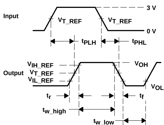
VOLTAGE WAVEFORMS
