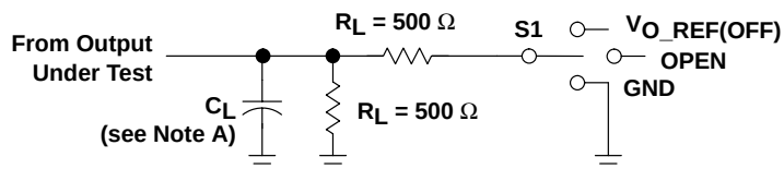
LOAD CIRCUIT for t_{pd} and t_{sk}
